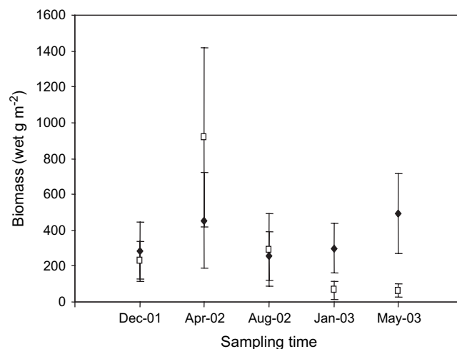
Fig. 4. Total macrobenthic community biomass (wet g m -2 ) in sediments from the central part of the Thau Lagoon (C4: full symbol) and near the shellfish farming zone (C5: open symbol), for the different sampling times. Data are mean \pm SD ( n = 3 ).
