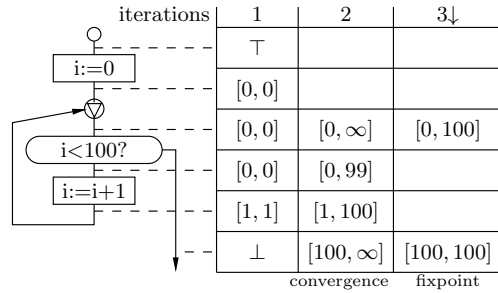
(a) A classical example where the decreasing sequence reaches the least fixpoint
