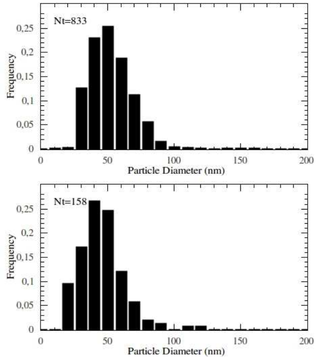
Figure 2: Histograms of the particle size in Mg-doped preform (top) and optical fiber (bottom).
