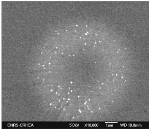
Figure 1: SEM picture of a Mg-doped fiber
