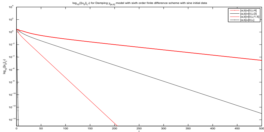
Figure 2: Norm L^2 for the damping \chi_{[a,b]} using a sixth order compact scheme.
