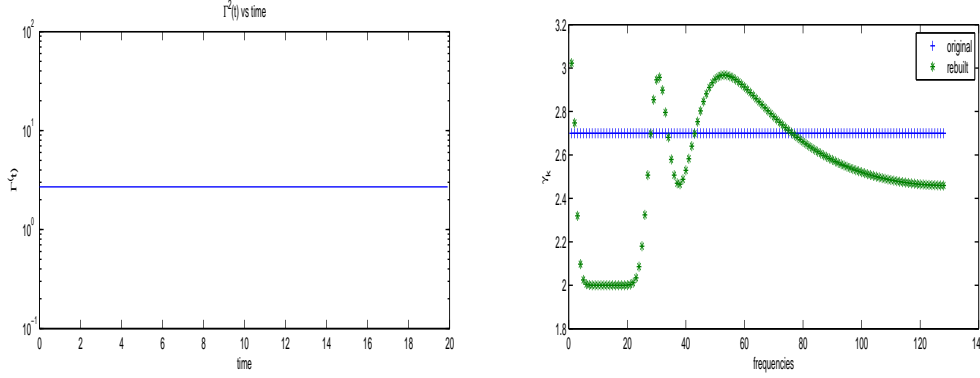
Figure 13: \Gamma^2(t) (left), comparison of the original and the rebuilt coefficients \gamma_k (right)
