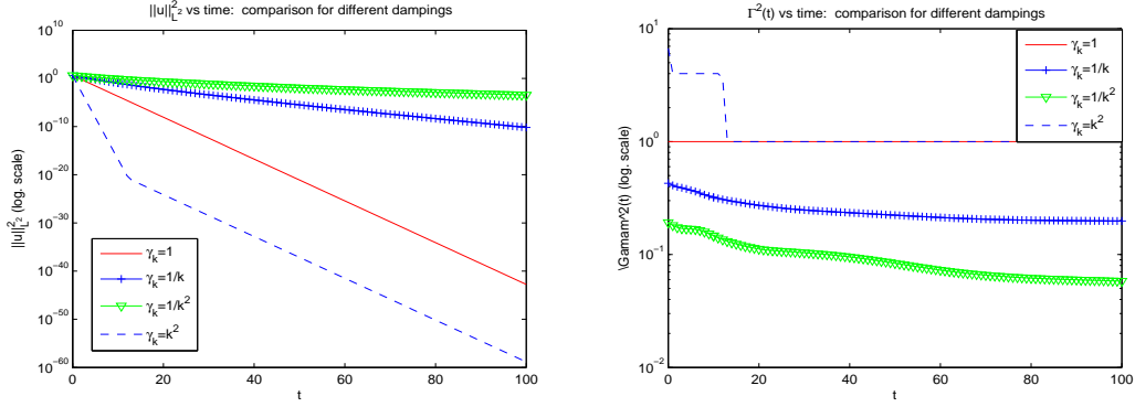
Figure 1: Comparison of L^2 -norm of the solution for different damping on [0, L] with L = 20 (left) and of \Gamma^2(t) (right).
