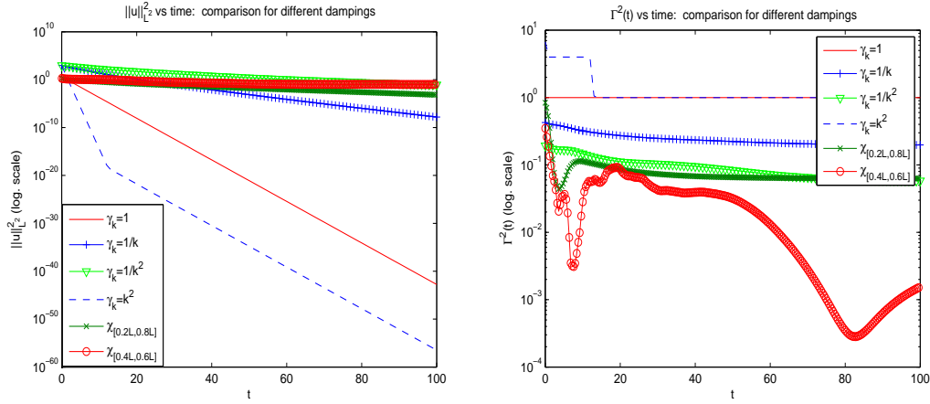
Figure 6: Comparison of the time evolution of L^2 -norm (left) and of \Gamma^2(t) (right) for the damping operators \mathcal{L}_\gamma and \chi_{[a,b]} on [0, L] with L = 20 .
