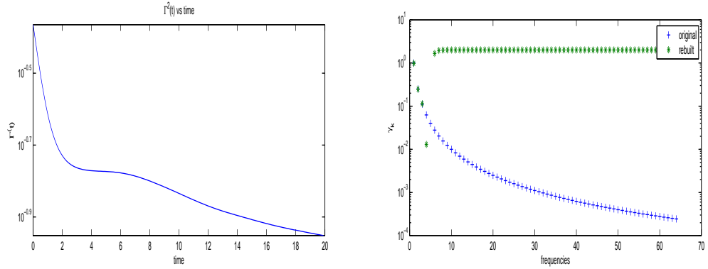
Figure 11: \Gamma^2(t) (left), comparison of the original and the rebuilt coefficients \gamma_k = \frac{1}{(|k| + 1)^2} (right)
