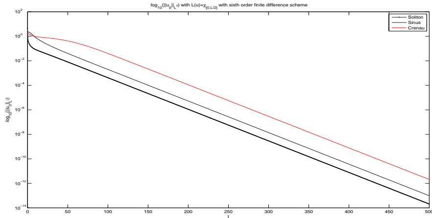
Figure 3: Norm |u|_{L^2} for the damping \chi_{[0,L/2]} using a sixth order compact scheme for initial data: S1 , S2 = \chi_{[0.5 \cdot L, 0.7 \cdot L]} et S3 .
