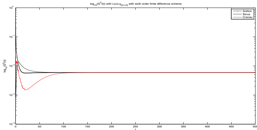
Figure 4: \Gamma^2(t) for the damping \chi_{[0,L/2]} using a sixth order compact scheme for initial data: S1 , S2 = \chi_{[0.5 \cdot L, 0.7 \cdot L]} et S3 .
