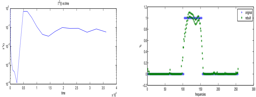
Figure 12: \Gamma^2(t) (left), comparison of the original and the rebuilt coefficients \mathcal{L} = \chi_{[0.4L, 0.6L]} (right)
