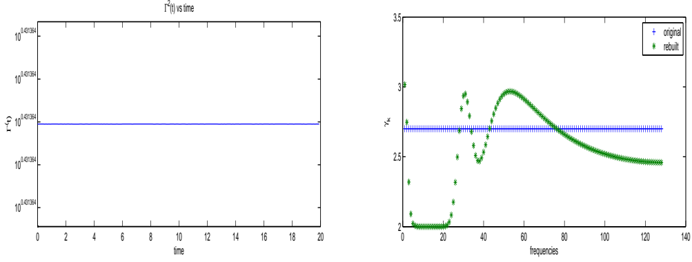
Figure 10: \Gamma^2(t) (left), comparison of the original and the rebuilt coefficients \gamma_k (right)
