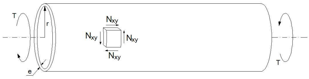
Figure 11. Hollow driveshaft subjected to an external torque 285x73mm (96 x 96 DPI)
