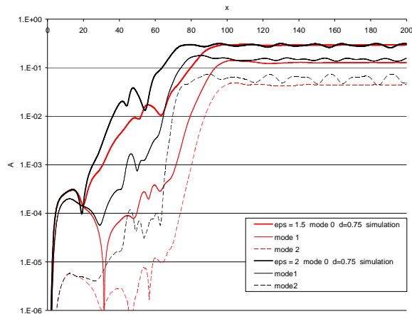
Figure 7. Influence of the Rayleigh number on the evolution of the temperature fluctuations along the channel. f = 0.23 .
