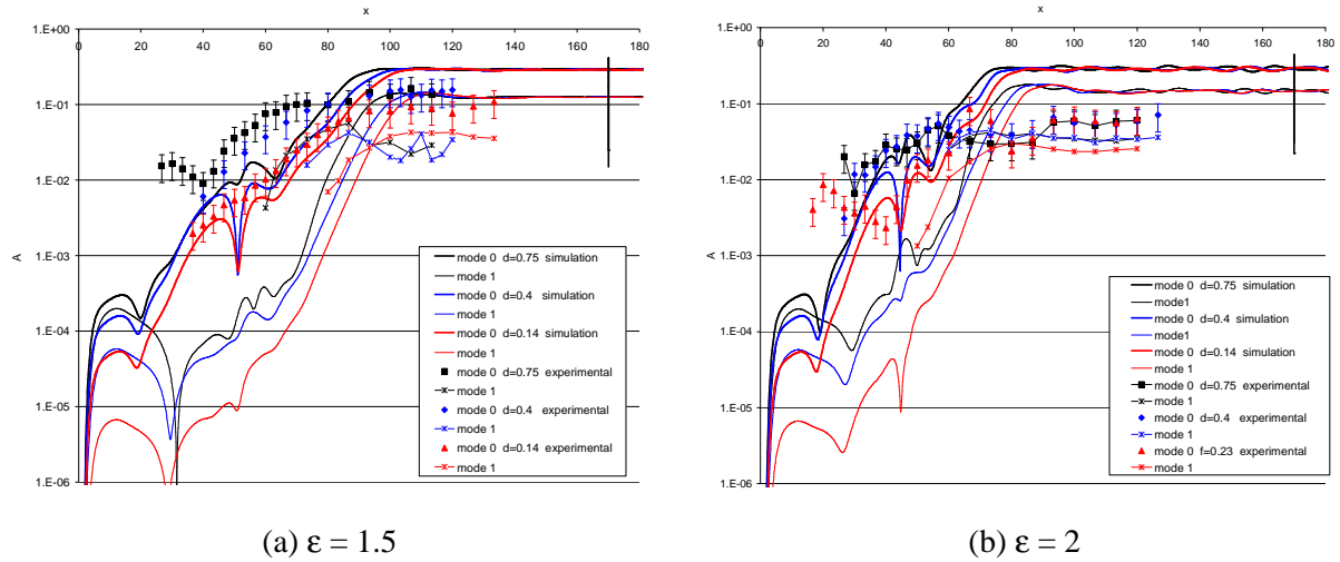
Figure 6. Influence of the excitation amplitude on the evolution of the temperature fluctuations along the channel: experimental and numerical results. f = 0.23 . d = 0.14 . The vertical bar at x = 170 indicates the variation range of the temperature fluctuation magnitude (fundamental mode) observed numerically when the transverse location, y , of the monitor point moves through the 5th roll (central part of the channel).
