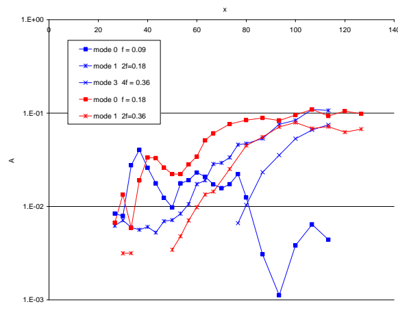
Figure 10. Evolution of the temperature fluctuations along the channel. Experiments. \epsilon = 1.5 , d = 1 , f = 0.09 and 0.18 .
