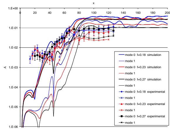
Figure 8. Influence of the forcing frequency on the evolution of the temperature fluctuations along the channel: experimental and numerical results. \epsilon = 2 , d = 0.14 .
