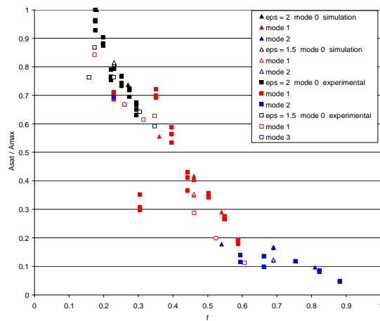
Figure 9. Influence of the forcing frequency on the normalized saturation amplitude. Comparison between experimental and numerical results.
