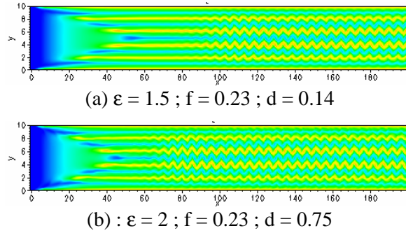
Figure 5. Instantaneous temperature field at channel mid-height resulting from periodic excitations at the inlet of the heated zone. The flow is coming from left to right. 10 rolls gradually develop from the inlet.
