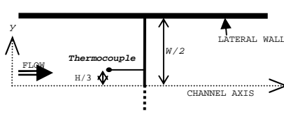
Figure 2. Location of the thermocouple in the horizontal plane at channel mid-height.
