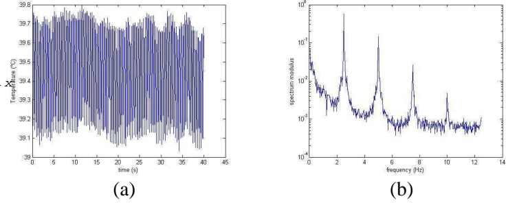
Figure 3. (a) Time evolution of the signal delivered by the thermocouple located at x = 120 , (b) modulus of the discrete Fourier transform (average over 10 samples). Forcing frequency f^* = 2.5 Hz, forcing amplitude d = 0.41 , Ra = 10000 , Re = 175 .
