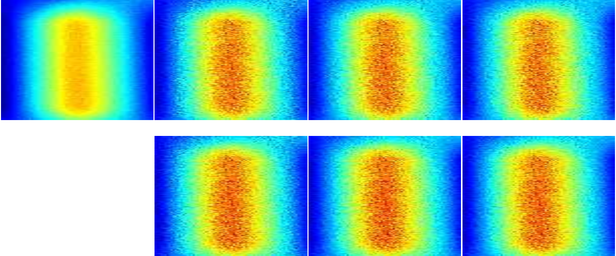
(b) Estimation in high irradiance range ( \sim 10^{4.4} ). Top row: Ground-truth, MLE, Kirk and Andersen, Robertson et al. Bottom row: Debevec and Malik, Mitsunaga and Nayar, Reinhard et al.
