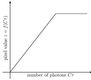
Figure 2.1: Camera response function for the linear + saturation model (raw data).
