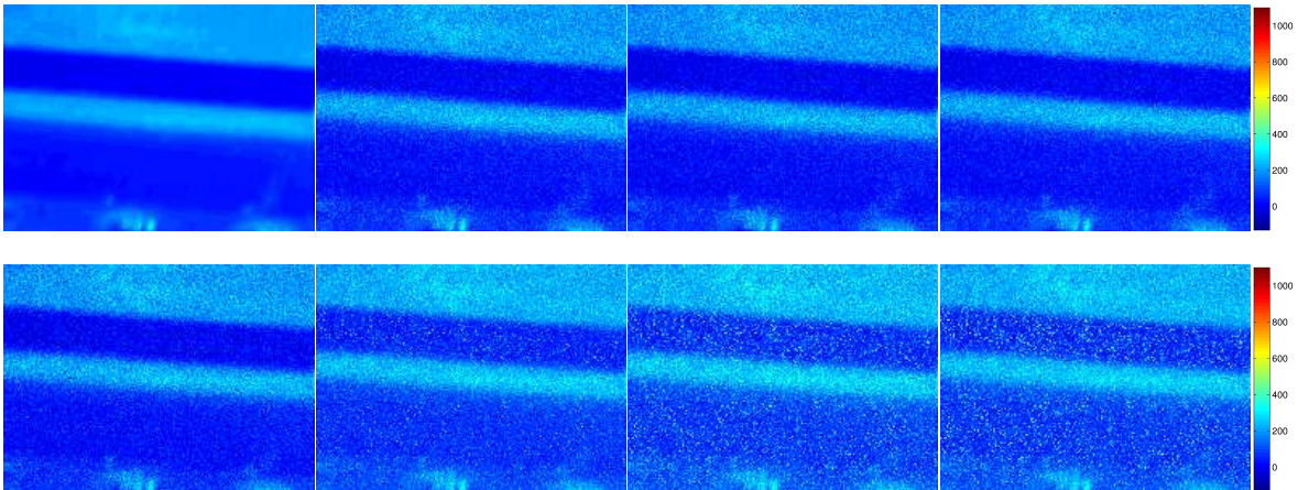
Figure 3.4: Synthetic data. Estimation in low-level irradiance range. Patch size 141 \times 193 . Top row: Ground-truth, MLE, Modified Kirk and Andersen, Robertson et al. Bottom row: Poisson, Debevec and Malik, Mitsunaga and Nayar, Reinhard et al. The results for MLE, Modified Kirk and Andersen, Robertson et al. and Poisson are quite similar and less noisy than those of Debevec and Malik, Mitsunaga and Nayar and Reinhard et al.
