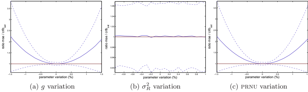
Figure 5.1: Dependence of the performance of the MLE estimator on the uncertainty in model parameters for Camera A (the results for Camera B are equivalent). A great dependence is found on both g and a . On the contrary, the variation for \sigma_R^2 is negligible.
