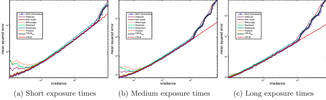
Figure 3.2: Comparison of the MSE curves and the CRLB for Camera A with 4 exposure times (results are similar for the other configurations). In all cases the MSE of the MLE is very close to the CRLB.
