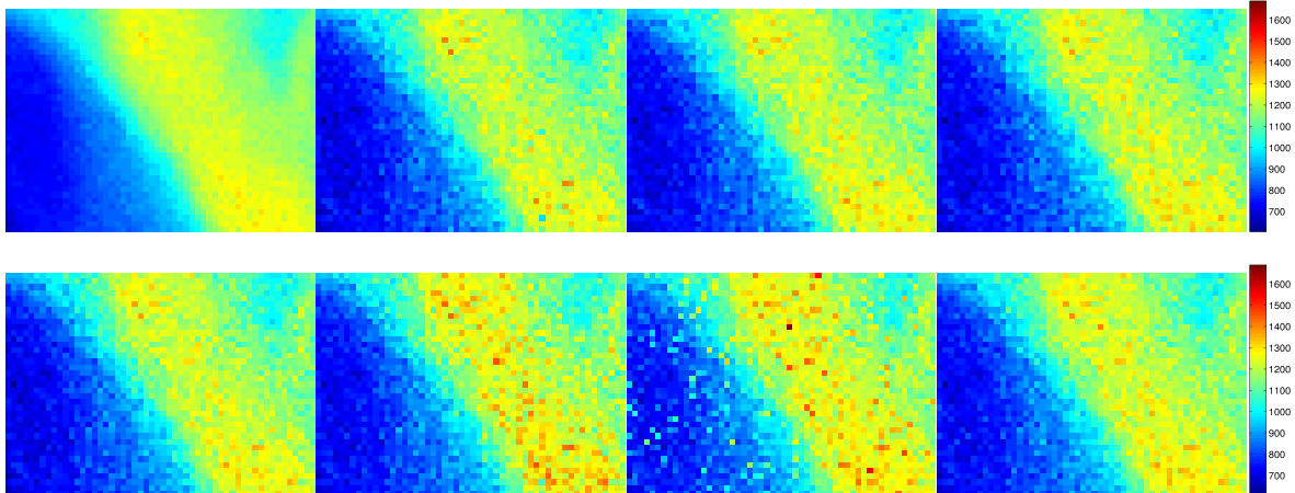
(b) Patch size 39 \times 54 . Top row: Ground-truth, MLE, Modified Kirk and Andersen, Robertson et al. Bottom row: Poisson, Debevec and Malik, Mitsunaga and Nayar, Reinhard et al.
