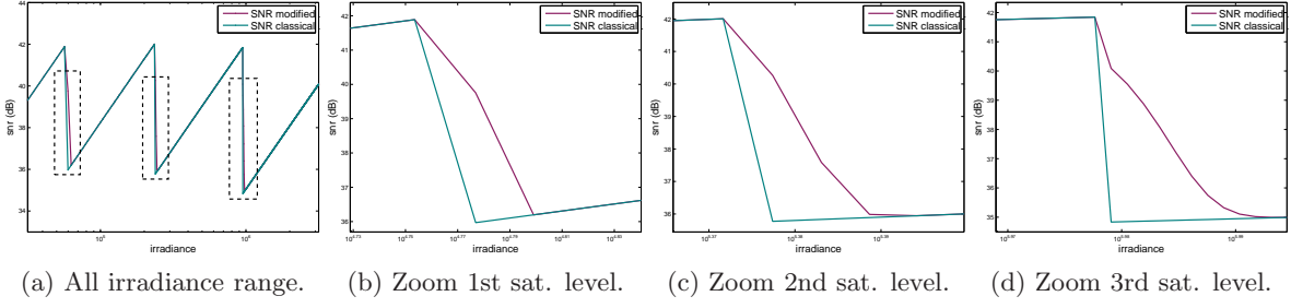
Figure 4.2: Comparison of the SNR obtained with the classical and the modified log-likelihoods. Both curves match except for the irradiance values in the transition between two saturation levels.
