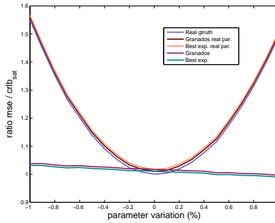
Figure 5.2: Dependence of the ground-truth computation with the uncertainty in model parameters. For small variations of the parameter the results of all computed ground-truths are almost equivalent. Yet for variations above 0.2% the performance announced by both ground-truths computed with the wrong parameters is highly superior than the real performance.
