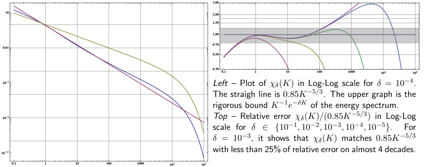
Figure 6: A striking observation : a logarithmic correction to the rigorous analytic estimates of the energy spectrum has a definite K^{-5/3} behavior on a large range of K .
