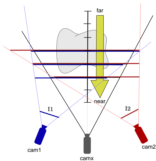
(a) Plane-sweeping algorithm : geometric configuration.
