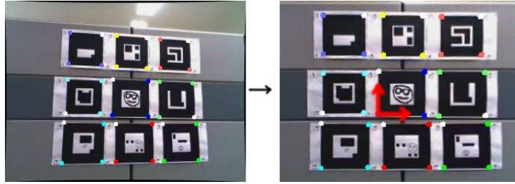
Fig. 3. Estimation of the relationship between every marker by homography.
