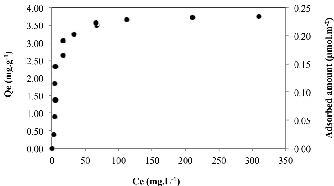
Figure 2. Adsorption isotherm of ADIBA onto the silica sol at 25^\circ\text{C} and \text{pH} = 9.1 . The experimental data are well fitted by the Langmuir adsorption model with a high correlation coefficient. The linearized form of the isotherm is shown in the Supporting Information (Figure S3). [\text{SiO}_2] = 50 \text{ g.L}^{-1} .
