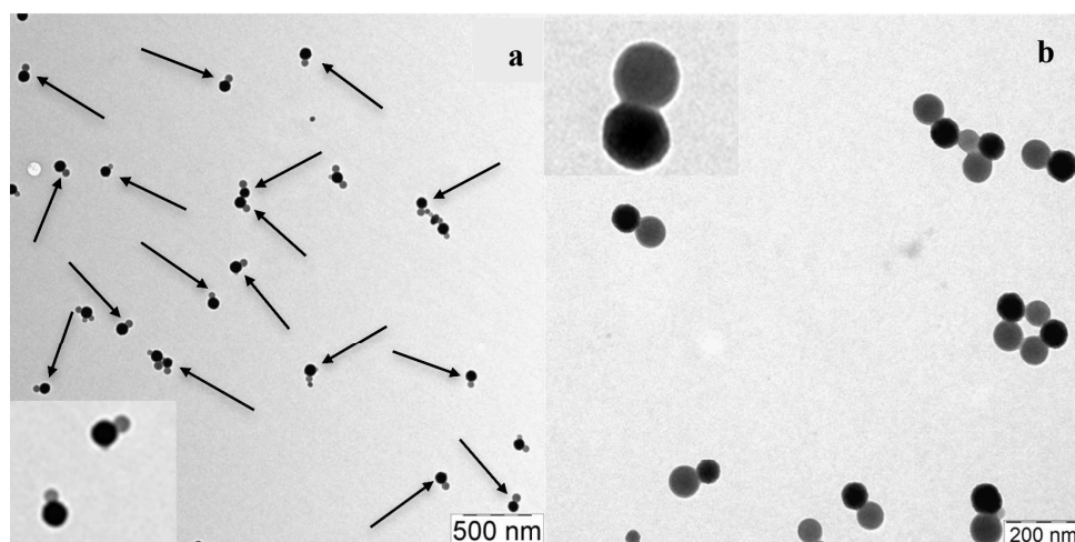
51 52 Figure 10. TEM images of dissymmetrical snowman-like (a) and dumbbell-like (b) silica/ 53 polystyrene composite particles. a) 13 % and b) 50 % conversion. Arrows point to the 54 dissymmetrical particles. [\text{SiO}_2] = 50 \text{ g}\cdot\text{L}^{-1} and NP30/SDS = 99/1 (entry 3 in Table 3). 55 56 57 58 59 60
