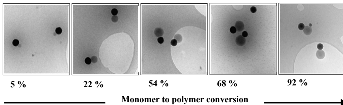
Figure 8. Evolution of particle morphology with conversion during the synthesis of dissymmetrical silica/PMMA heterodimers. [\text{SiO}_2] = 40 \text{ g.L}^{-1} and NP30/SDS = 98/2 (wt/wt) (entry 10 in Table 2).
