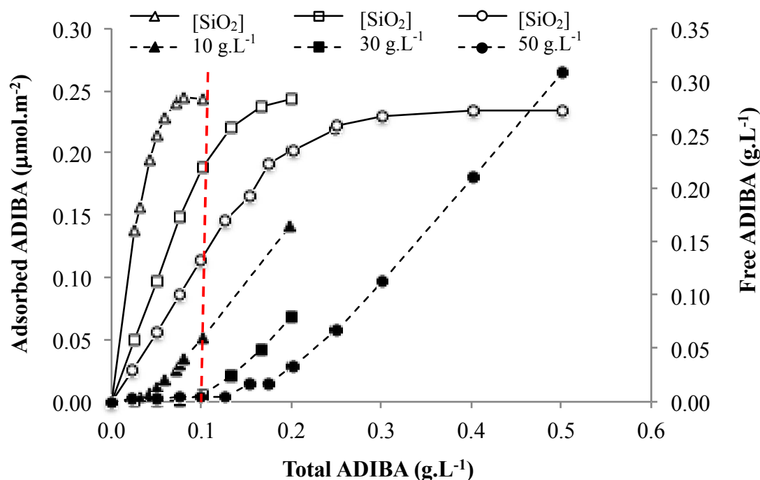
Figure 3. Langmuir isotherm data plotted as the amount of adsorbed ADIBA against its initial concentration in water (open symbols) for silica concentrations of 10, 30 and 50 g.L -1 , respectively. The filled symbols represent the evolution of the ADIBA equilibrium concentration in water as a function of the initial ADIBA concentration.
