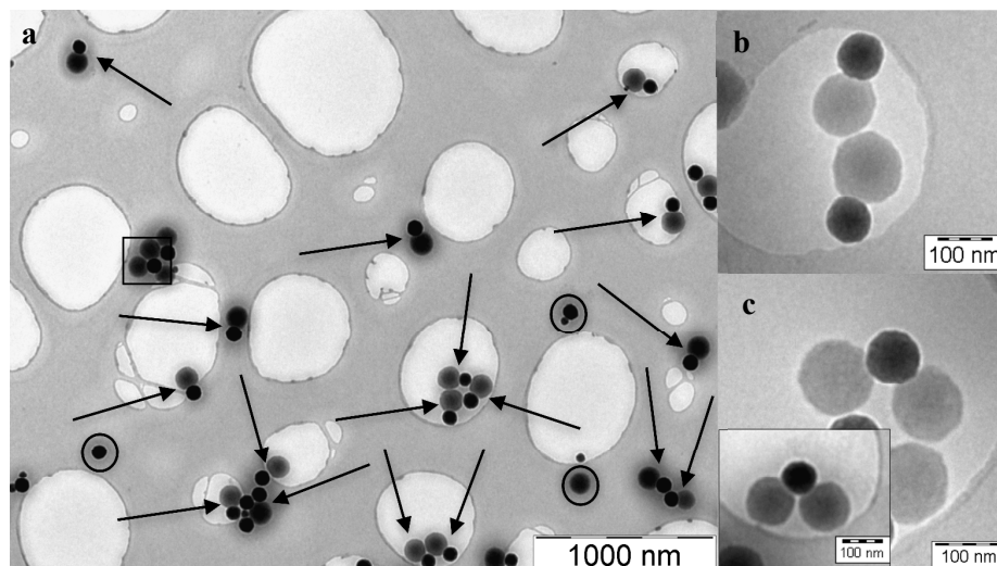
Figure 7. Cryo-TEM images of: a) dissymmetrical silica/PMMA heterodimers with a N_{\text{Latex}}/N_{\text{Silica}} ratio of 0.95 (monomer conversion = 92 %) showing the presence of dumbbell-shaped particles (arrows), trimers (squares) and isolated silica (circles). b) and c) correspond to an enlarge view of respectively the dumbbell and trimer particles. [\text{SiO}_2] = 40 \text{ g.L}^{-1} and NP30/SDS = 98/2 (wt/wt) (entry 9 in Table 2).
