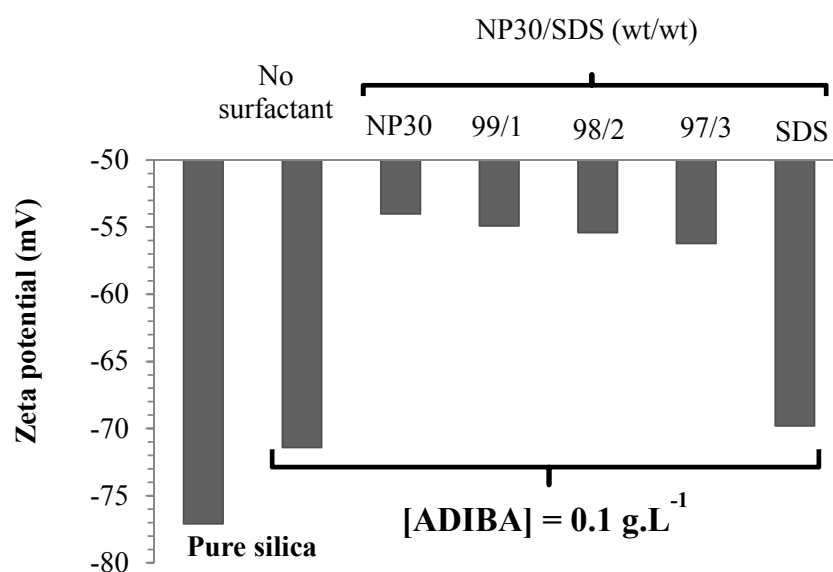
Figure 5. Electrophoretic measurements of the aqueous silica sol before ADIBA adsorption, after ADIBA adsorption ( [ADIBA] = 0.1 \text{ g.L}^{-1} ), and after adsorption and addition of NP30/SDS mixtures of various compositions. [Silica] = 50 \text{ g.L}^{-1} . \text{pH} = 9.1 .
