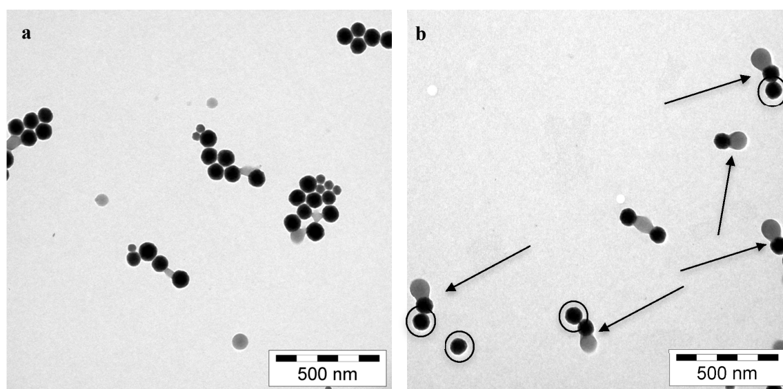
38 39 40 41 42 43 44 45 46 47 Figure 1. TEM images of silica/PMMA nanocomposite latexes synthesized using a) a non-ionic (VA86) and b) a cationic (ADIBA) initiator (entries 1 and 2 in Table 2). Arrows point to the silica/PMMA dissymmetrical particles. Black circles show isolated silica particles.
