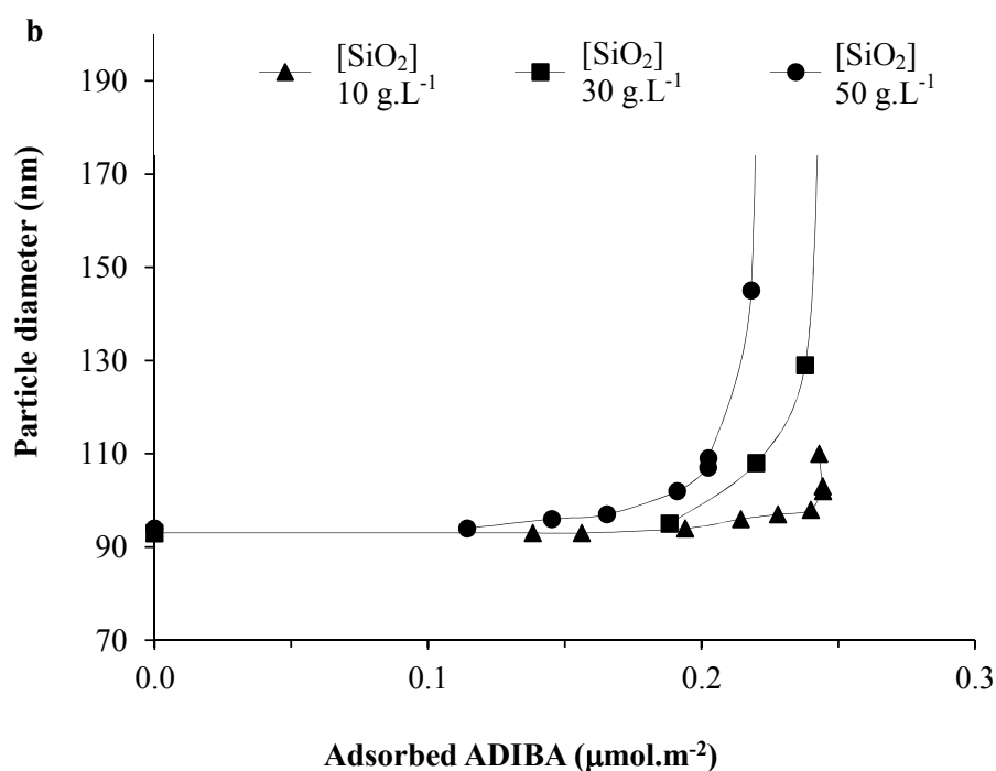
Figure 4. Effect of ADIBA adsorption on colloidal stability of the silica sol. The silica particle diameter is plotted against: a) the overall initial ADIBA concentration in water, and b) the ADIBA adsorbed amount ( \mu\text{mol.m}^{-2} ) for various silica concentrations.
