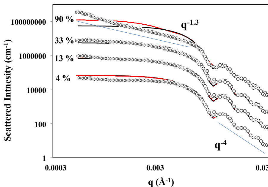
25 26 27 28 29 30 31 32 33 34 35 36 37 38 39 40 41 42 43 44 45 46 47 48 Figure 9. I(q) versus q plots during the synthesis of silica/PMMA dissymmetrical latex 49 50 particles. The full lines in black are the predicted scattering intensity of the silica spheres while 51 52 the dotted lines in red correspond to that of the silica/PMMA heterodimers. [\text{SiO}_2] = 50 \text{ g.L}^{-1} and 53 54 \text{NP30/SDS} = 98/2 (entry 2 in Table 2). 55 56 57 58 59 60
