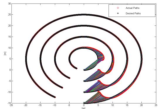
Fig. 3. Coordinated path following in in-line formation.
