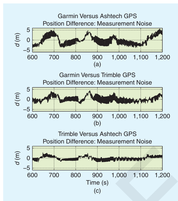
Figure 5. The measured distance error between different GPS receivers. (a)–(c): Garmin versus Ashtech, Garmin versus Trimble, and Trimble versus Ashtech.
