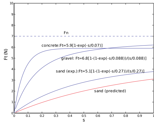
Fig. 15. Data interpolation for several soils
