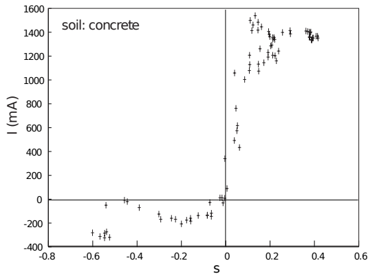
Fig. 13. Slip-current relation
