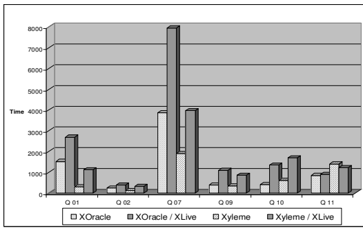
Figure 3 : Benchmarking (Oracle, Xyleme, XLive)
