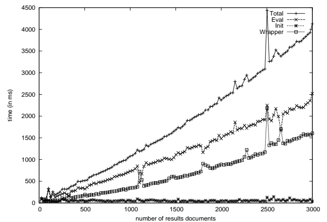
Figure 3: Execution time for each step
