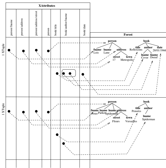
Figure 2: Example of an XRelation
