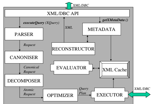
Figure 1: Overview of the mediator architecture
