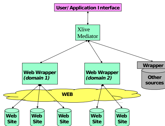
Figure 2. Web wrappers using domain view in mediation architecture
