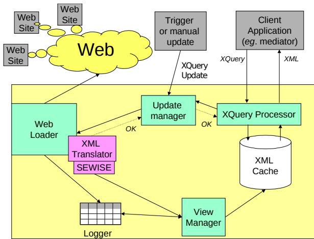
Figure 3. XQuery view architecture
