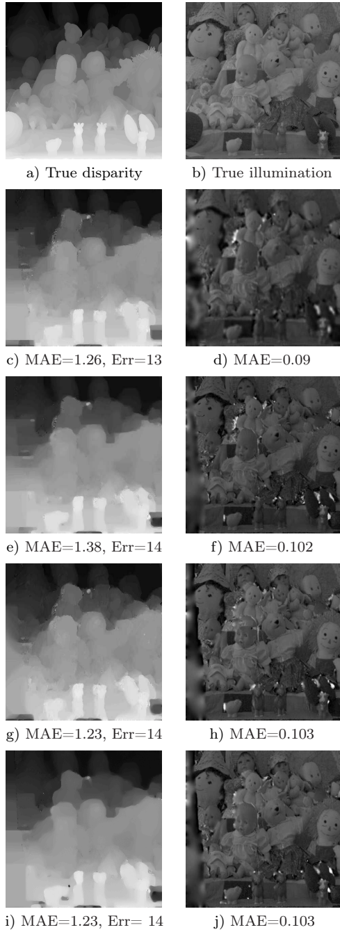
Fig. 4 Results for Dolls stereo pair: proposed approach considering for c)-d)- \ell_1 -cost and S_1 \cap S'_2 with (u_{\min}, u_{\max}) = (20, 75) , (v_{\min}, v_{\max}) = (0.1, 1.1) , (\tau'_2, \kappa_2) = (92000, 230) , e)-f)- \ell_4 cost and S_1 \cap S'_2 , g)-h) \ell_1 cost and S_1 \cap S_2 \cap S_3 with (\tau_2, \kappa_2) = (34000, 230) , (\tau_3, \kappa_3) = (180000, 570) , i)-j)- \ell_{3/2} cost and S_1 \cap S_2 \cap S_3 .
