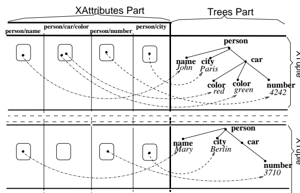
Figure 2: XTuple.
