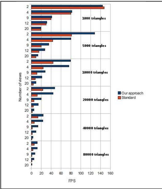
Figure 7. Performances of our approach compared to the standard one. Tests are applied with various numbers of views and triangles.
