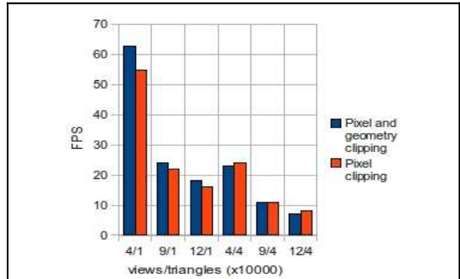
Figure 9. Comparison of the frame rate between a clipping in pixel shader stage and a clipping in geometry and pixel shader stages.
