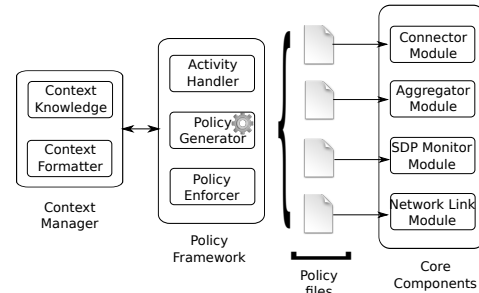
Fig. 4. XTalk Modules
