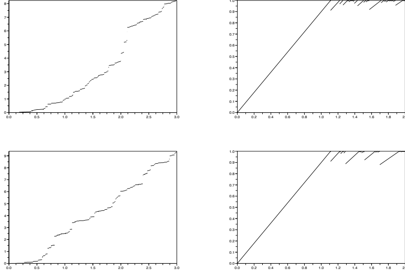
FIGURE 1. Two sample paths of the stochastic process M built using the function \gamma(y) := \min(1/2 + y/4, 0.9) . On the right hand-side are plotted the theoretical spectra D_M([0, 3], \cdot) .
