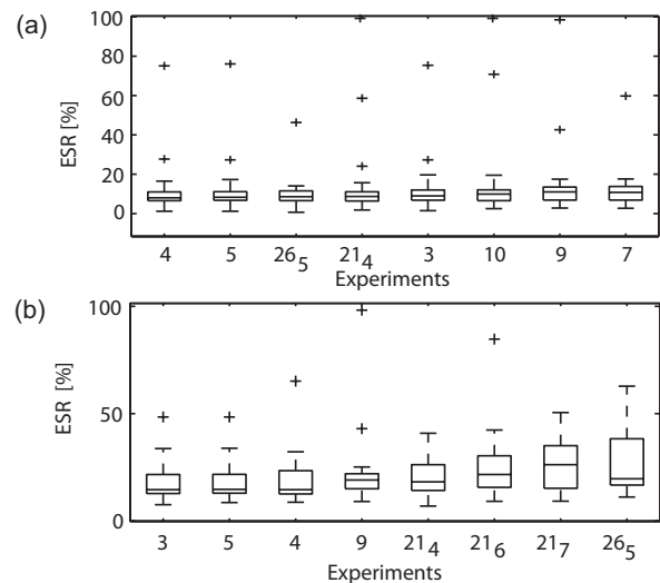
Fig. 12. Statistical performance of the ESR for cross validation of model parameters when they are identified with the new DoE and classical Experiment # 3. (a) shows the results for modified SP model and (b) shows VMax model. The horizontal axis shows the DoE . The vertical axis shows the ESR when the model estimates the f MR .
