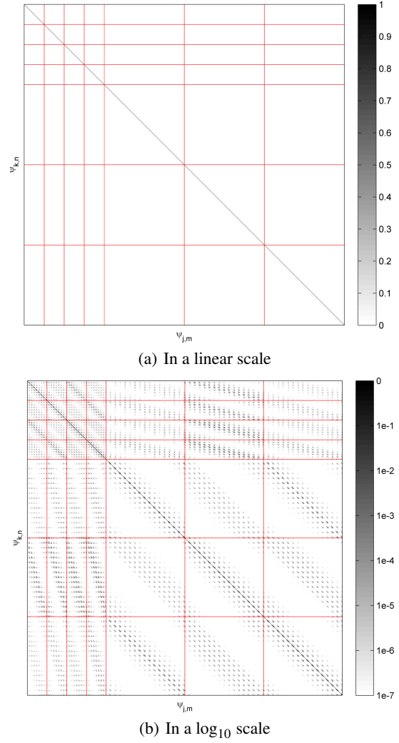
FIGURE 3 – Matrix \Theta for the variable operator illustrated in Figure 2. This matrix is obtained using Daubechies 8 wavelets and a decomposition level J = 2 .
