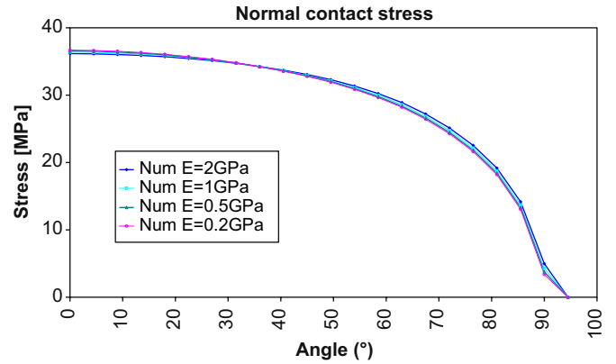
Fig. 12. Normal contact stress on the bolt-ring surface for the case R_2 = 30 mm.
