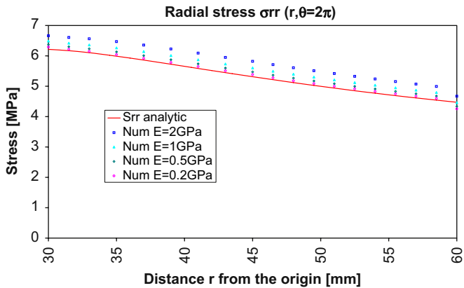
Fig. 10. Radial stress component \sigma_{rr}(r, \theta = 2\pi) with R_2 < r < R_3 ( R_2 = 30 mm).
