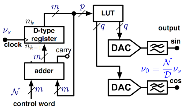
Figure 1. DDS scheme.
