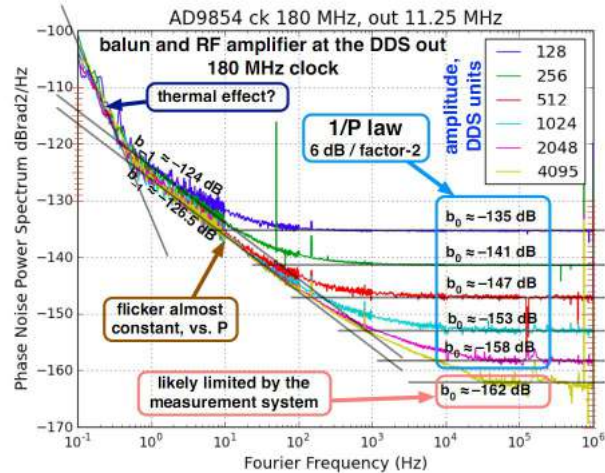
Figure 8. AD9854 phase noise measured at different output amplitudes
