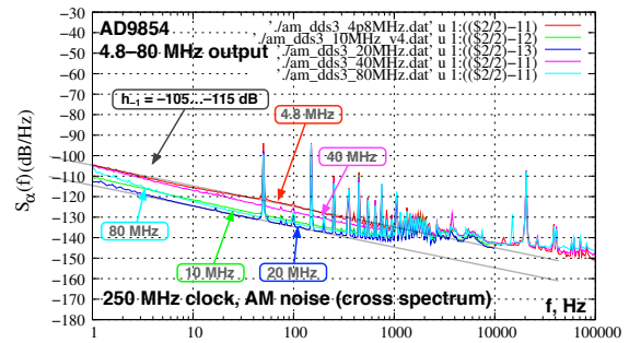
Figure 16. AM noise of the AD9854.
