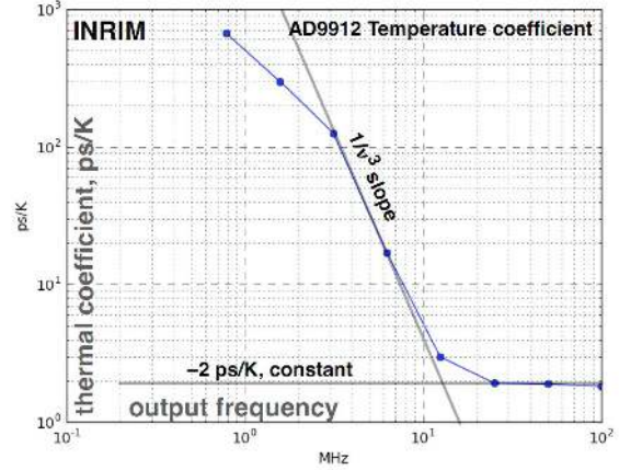
Figure 12. Thermal coefficient of the AD9912 vs. the output frequency.
