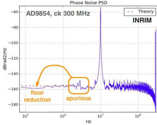
Figure 4. A simulation shows a reduction in the noise floor related to the presence of some spurs.
