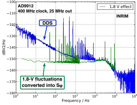
Figure 11. The supply-voltage noise impacts on the DDS phase noise.
