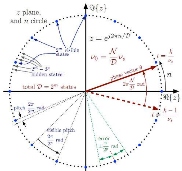
Figure 2. DDS state variable, and its relationships to the output phase.
