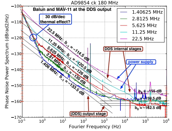
Figure 5. AD9854 phase noise measured at different output frequencies.
