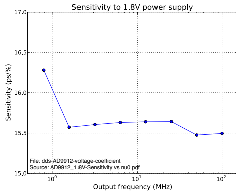
Figure 10. Power-supply rejection of the AD9912 1.8 V line, measured by switching the supply voltage by \pm 5\% around the nominal value.
