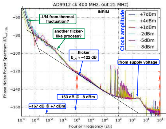
Figure 14. AD9912 phase noise spectrum measured at 400 MHz clock for a few values of the clock amplitude. The amplitude is given in dBm on a 50 \Omega resistance, 0 dBm is 224 mV.
