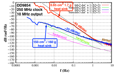
Figure 13. Effect of the heat sink on the phase noise spectrum.
