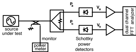
Figure 15. Scheme for the measurement of AM noise.
