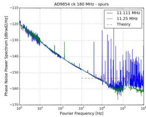
Figure 9. Phase noise spectra with a small change in the control word.
