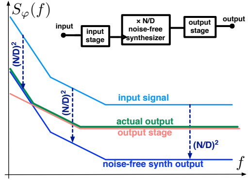
Figure 3. Phase noise model for a frequency synthesizer.
