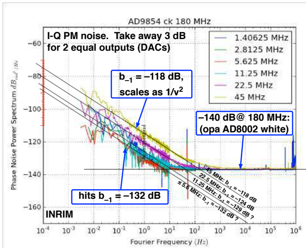
Figure 7. Phase noise of the output stage, measured by comparing the phase difference between the I output and the Q output.
