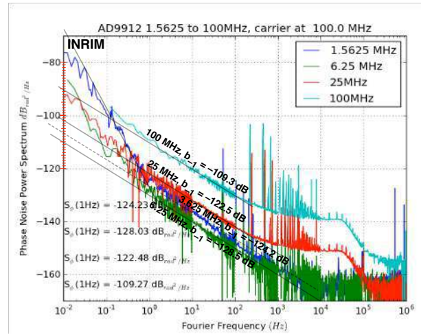
Figure 6. AD9912 phase noise measured at different output frequencies.
