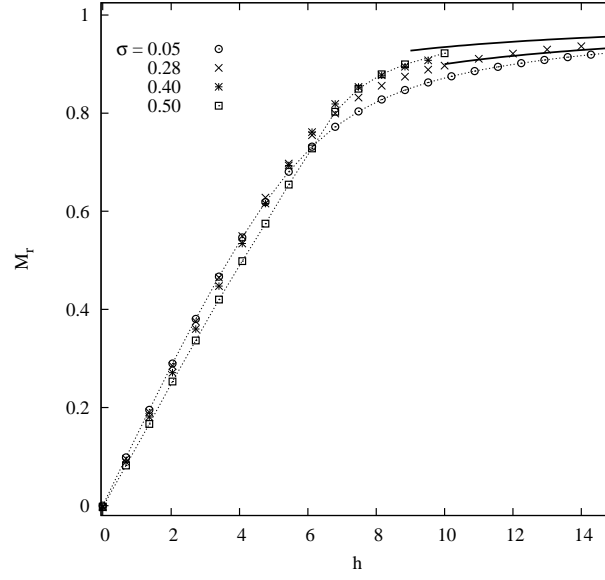
Figure 7: Magnetization in terms of the applied field for different values of the \ln(d) standard deviation \sigma and d_m/d_{ref} = 1.33 , \Delta/d_{ref} = 0.20 and \beta^* = 1.0 . N_p = 1007 ( \sigma = 0.05 ), 923 ( \sigma = 0.28 ); 985 ( \sigma = 0.40 ) and 990 ( \sigma = 0.50 ). The dotted lines are guides to the eye. The solid lines are the asymptotic limits for \sigma = 0.05 (bottom) and \sigma = 0.50 (top).
