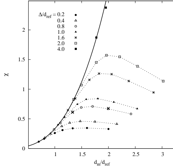
Figure 4: Linear susceptibility in terms of the median size d_m/d_{ref} for different values of the coating layer thickness \Delta in the quasi monodisperse case, \sigma = 0.05 and \beta^* = 1.0 . The two crosses on the \Delta/d_{ref} = 0.8 curve correspond to the direct calculation without using the scaling transformation (6). The dotted lines are guides to the eye and the solid line corresponds to the non interacting case.
