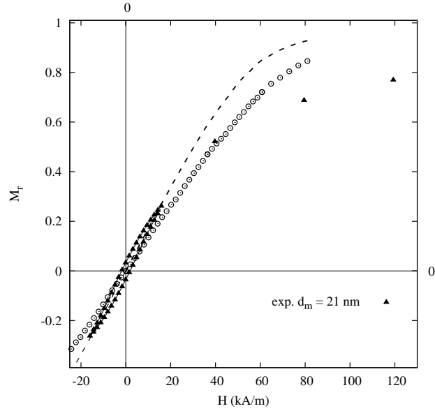
Figure 14: Comparison between MC simulations and the experimental magnetization curve at room temperature for d_m = 21 nm. The simulations are performed with d_m = 20 nm, \beta^* = 1 , N_p = 998 , \epsilon_K^{(0)} = 2.38 (open circles) or 1.19 (dashed line).
