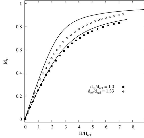
Figure 9: Magnetization curve with the anisotropy energy \epsilon_K^{(0)} = 2.38 , \sigma = 0.05 and the particles sizes as indicated. The solid lines correspond to \epsilon_K = 0 , \beta^* = 1 and N_p = 1007 .
