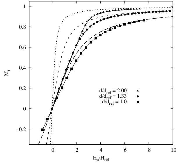
Figure 6: Magnetization in terms of the applied field for different values of the median diameter, \Delta/d_{ref} = 0.20 , \beta^* = 1.0 and N_p = 1007 in the quasi monodisperse case, \sigma = 0.05 . The corresponding non interacting curves (diameter distribution weighted Langevin curves) for d_m/d_{ref} = 1.0 (long dash), 1.33 (short dash) and 2.0 (dotted line) are displayed for comparison.
