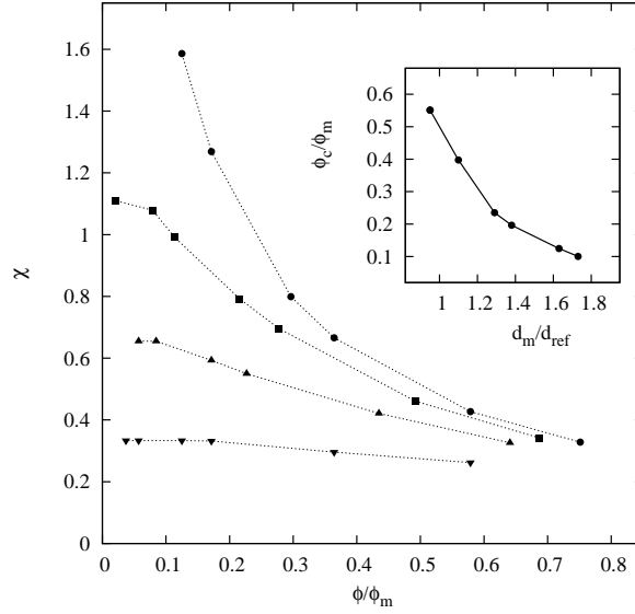
Figure 5: Susceptibility \chi in terms of the reduced volumic fraction, for \sigma = 0.05 , \beta^* = 1.0 , and d_m/d_{ref} = 2.0 (solid circles); 1.50 (solid squares); 1.25 (upward triangles) and 1.0 (downward triangles). \varphi_m = \varphi(\Delta = 0) . In the present work \varphi_m \simeq 0.59 . Inset: reduced critical volumic fraction defined as \chi(\varphi, \epsilon_d)/\chi(\epsilon_d = 0) = 0.80 in terms of the median particle size.
