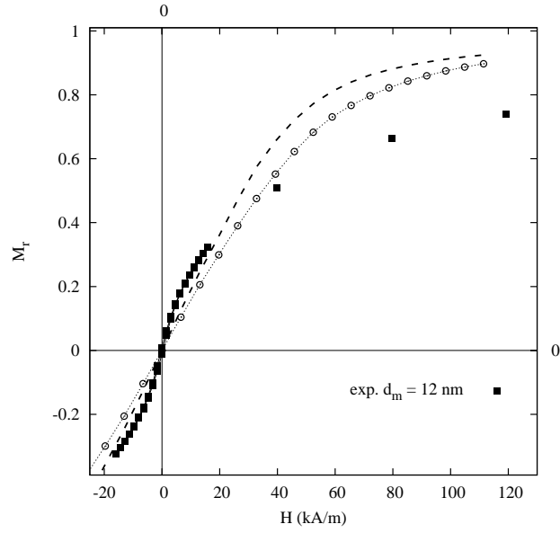
Figure 13: Comparison between MC simulations and the experimental magnetization curve at room temperature for d_m = 12 nm. The simulations are performed with \beta^* = 1 , N_p = 980 , \epsilon_K^{(0)} = 2.38 (open circles) or 1.19 (dashed line). The dotted line is a guide to the eye.
