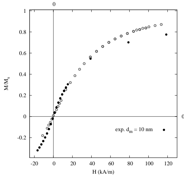
Figure 12: Comparison between MC simulations and the experimental magnetization curve at room temperature for d_m = 10 \text{ nm} . The simulation are performed with \beta^* = 1 , \epsilon_K^{(0)} = 2.38 and N_p = 923 .
