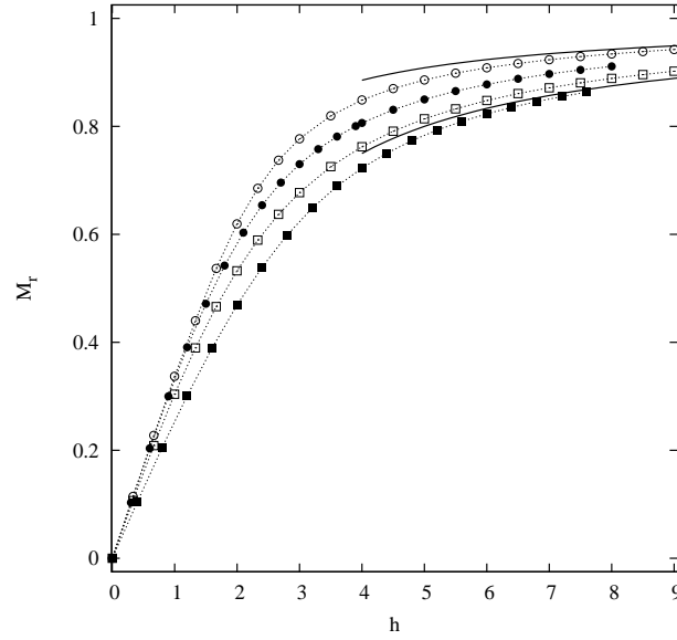
Figure 8: Magnetization in terms of the applied field for \sigma = 0.05, 0.20, 0.28 and 0.40 from bottom to top. and d_m/d_{ref} = 1.00 , \Delta/d_{ref} = 0.20 , \beta^* = 1.0 . The dotted lines are guides to the eyes and the solid lines are the corresponding asymptotic limits for \sigma = 0.05 and \sigma = 0.40 .
