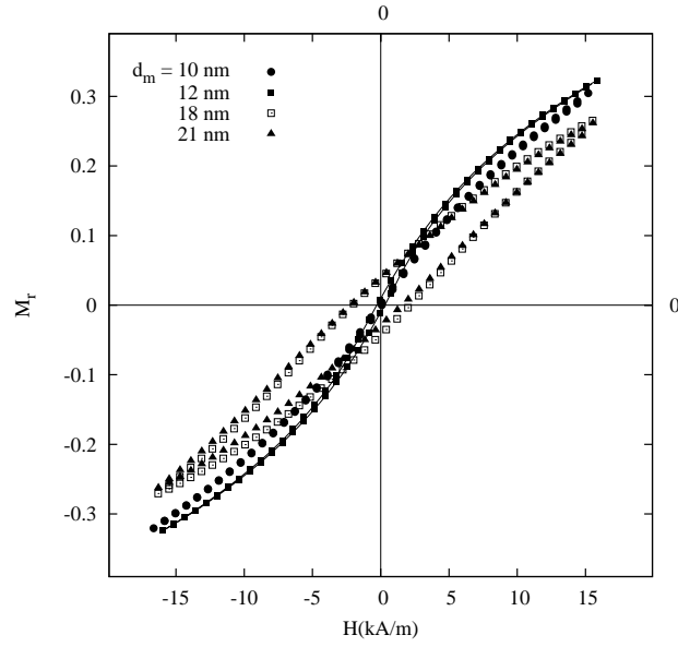
Figure 11: Experimental low field magnetization curves at room temperature for powder samples of \gamma - \text{Fe}_2\text{O}_3 from ref. [24] with polydispersity \sigma \simeq 0.26 and median sizes as indicated.
