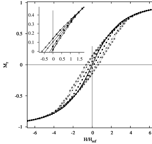
Figure 10: Magnetization curve with the anisotropy energy \epsilon_K^{(0)} = 2.38 , d_m/d_{ref} = 1.33 and \beta^* = 1 in the polydisperse case with \sigma = 0.35 (open circles); 0.28 (triangles); 0.20 (squares) compared to the quasi monodisperse case, \sigma = 0.05 (solid line). Insert: detail of the downward magnetization curve in the vicinity of h = 0 , showing the evolution of the remanence and coercivity with \sigma for \sigma = 0.35, 0.28, 0.20 and 0.10 (open squares) from top to bottom.
