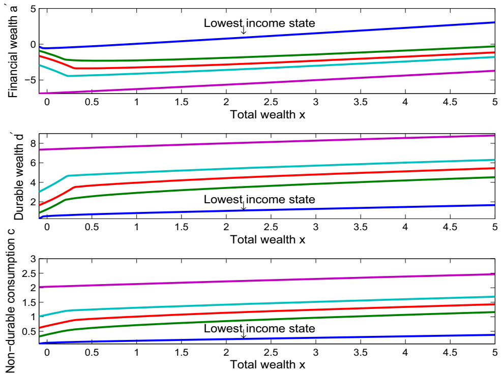
Figure 2: Policy functions without adjustment costs ( \alpha = 0 ) for the five income states, conditional on d = 0.05 , plotted for total wealth x \leq 5 .
