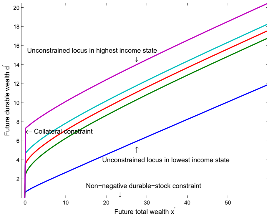
Figure 1: The relationship between future total wealth and future durable wealth for five different income states without adjustment costs.
