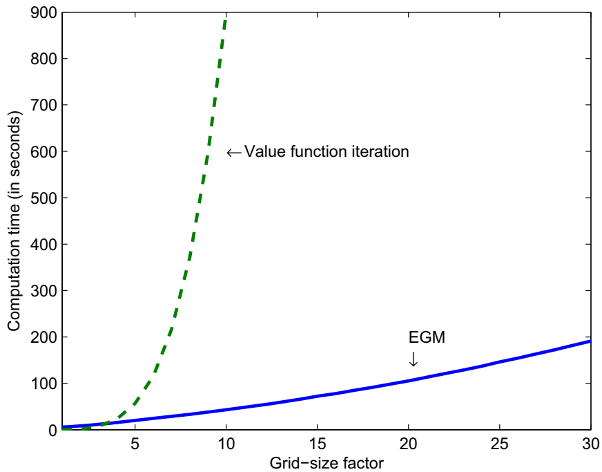
Figure 3: Computation time of the model without adjustment costs, as a function of the grid size. Notes: Solid graph: computation time for the EGM; dashed graph: computation time for discretization with value function iteration. A grid-size factor of 10 means twice as many gridpoints for x' and twice as many points for d than for a grid-size factor of 5.
