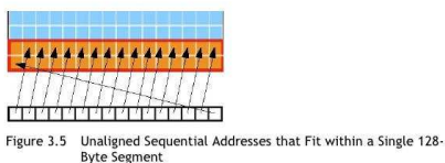
FIGURE 7. Schematic of data coalescence, extracted from the “CUDA C Best Practices Guide”, NVIDIA 2012 [1]
