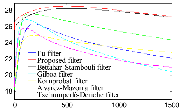
Fig. 9. PSNR representation of Face image as a function of the number of iterations.
