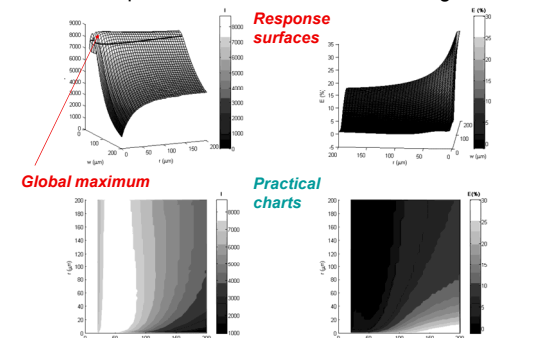
Fig 4. Response surface of the performance index I representing the area under the sound absorption curve in the frequency range 0 - 10 000 Hz for varying (w-throat size, r-fiber radius) couples (top-left); and associated 2D practical chart (bottom-left). Response surfaces of the error E made on I when using the simplified model instead of the refined one (top-right); and corresponding practical chart (bottom-right).
