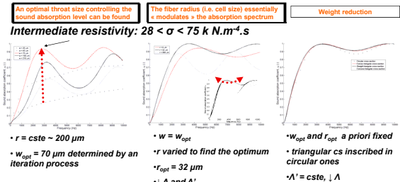
Fig 3. Throat size (left), fiber radius (center), and cross-section shape (right) effects. This section reports and quantifies differences obtained with the simplified and refined models, see Fig. 4.
