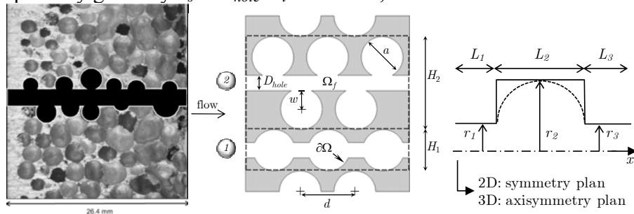
Figure 1. Example of a perforation through a real closed-cell aluminum foam sample (left). Two-dimensional model geometry of a perforated closed-cell metallic foam (center), showing two periodic unit cell (PUC) configurations: (1) lined-up, and (2) alternated.
