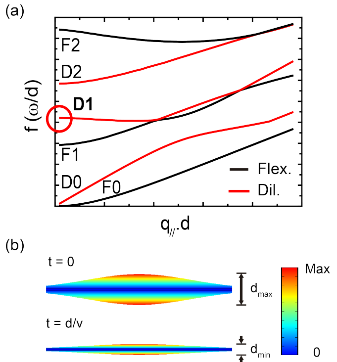
Figure 1. (a) Dispersion relation of a free-standing silicon membrane, showing flexural ( ) and dilatational ( ) modes. The mode primarily excited by the pump pulse is the first-order dilatational mode at zero parallel wavevector, D_{q_{\parallel}=0}^1 . (b) Schematic diagram of the displacement field of the excited mode calculated by finite element simulations. The change in thickness d due to the oscillation of the D_{q_{\parallel}=0}^1 mode is of the order of 1 pm and below, with a corresponding change in reflectivity of the order of 10^{-5} .
