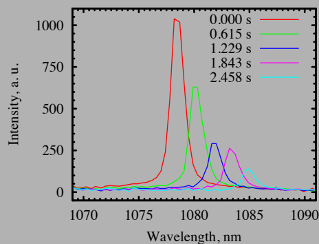
Video recording of the time drift of the laser wavelength of the Fabry-Perot fiber laser for pump power of 0.8 W. The video was captured by the CCD-type spectrometer (video is available on-line).
