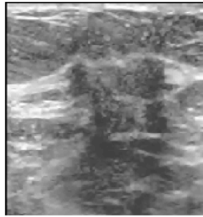
(c) SigShrink _{\pi/6, \lambda_m}
