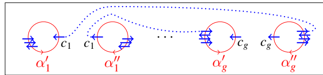
Figure 3: Rectangular diagram of (\mathcal{D}, \mathfrak{m}, w)
