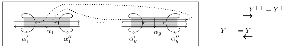
Figure 19: The punctured surface H_{a,2}^m
