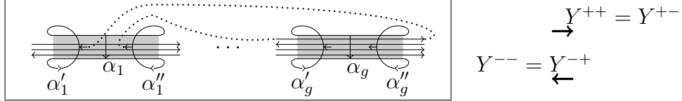
Figure 15: The punctured surface H_{a,2}^P
