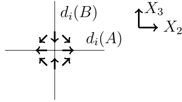
Figure 9: Projection of X
