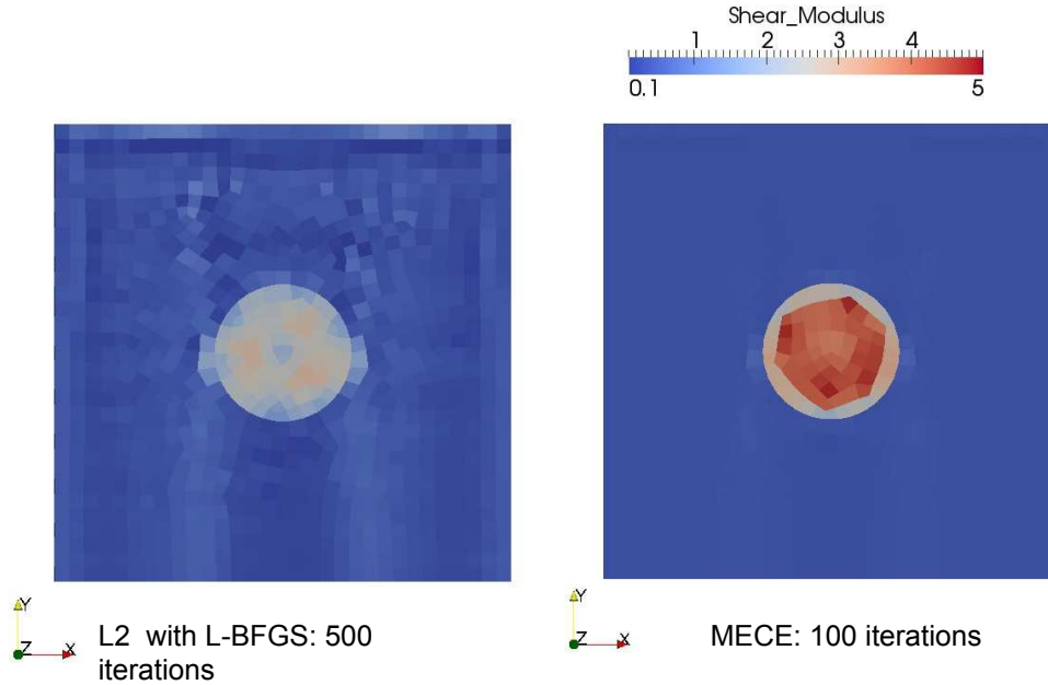
Figure 10: Comparison between MECE and L^2 /BFGS: solutions. Units: Pa.
