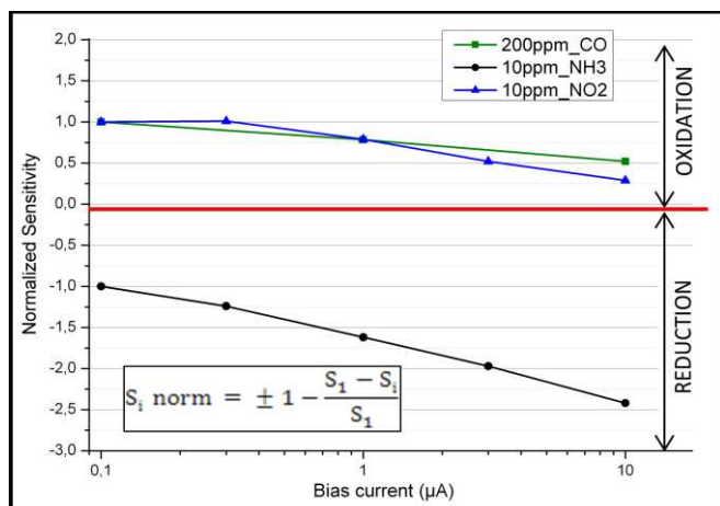
Figure 7. Normalized sensitivities of WO 3 sensitive layer to three different gases
