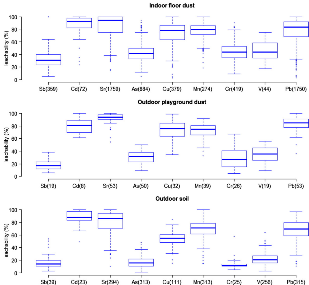
Fig. 1. Metal leachability (unweighted by sampling weights) in dwellings (indoor dust) and playgrounds (outdoor soil or dust) of children. France 2008–2009.
