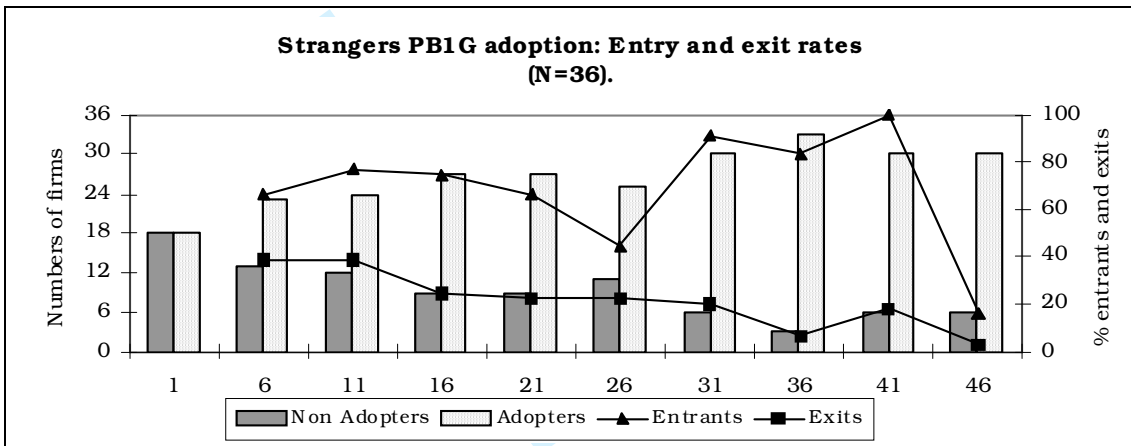
Figure 8: PB1G-S adoption patterns
