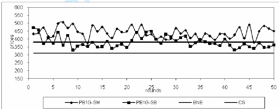
Figure 5: Evolution of average per round effective prices, PB1G-SM and PM1G-SB.
