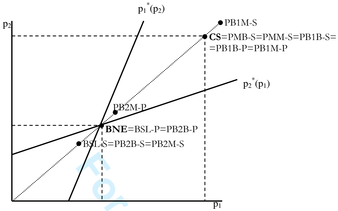
Figure 12: Summary of average effective prices
