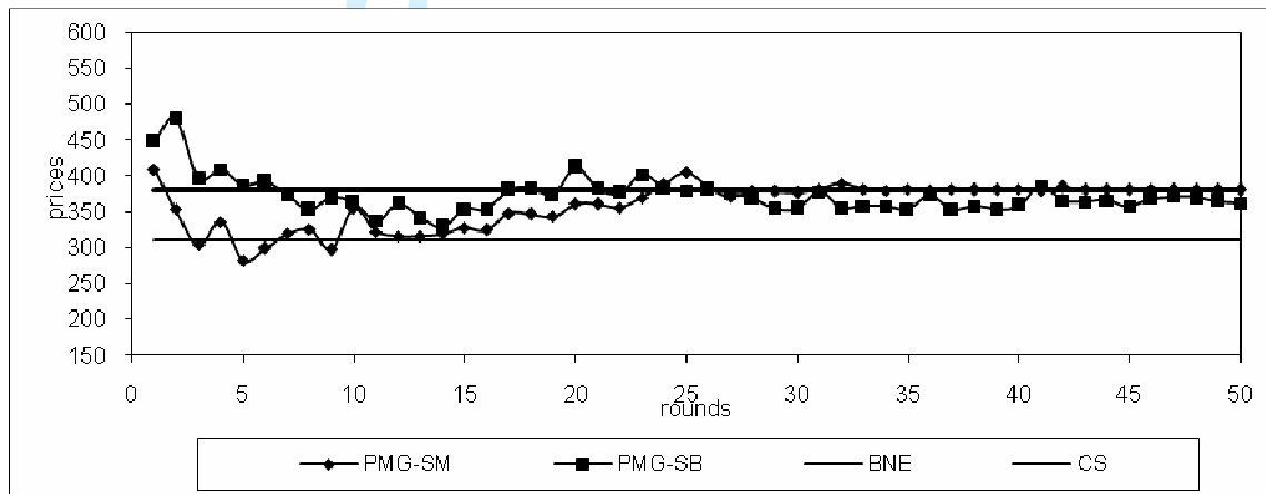
Figure 2: Evolution of average per round effective prices, PMM-S and PMB-S.
