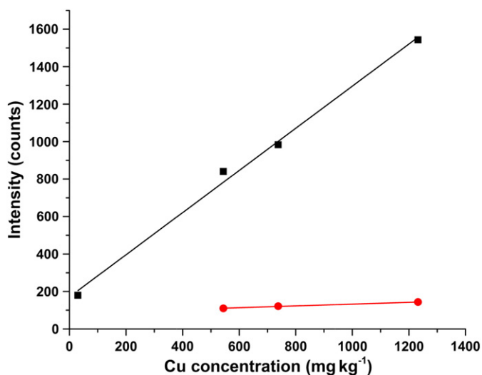
Fig. 2. Calibration curves of Cu for MA-LIBS (black squares) and the traditional LIBS (red circles).
