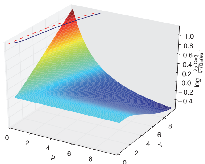
FIG. 6. Difference of the bulk pressure as a function of the parameters \gamma and \mu . Contour line where \lambda_0(Q=0) = \lambda_0(Q=0.5) (blue solid line) compared with the approximate transition line (65) (red dashed line).
