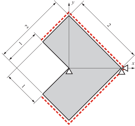
Figure 17: Problem 3. L-shaped domain.
