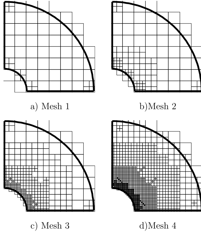
Figure 4: Problem 1.a. Sequence of h -adapted meshes for the mean radial displacement along \Gamma_o .
