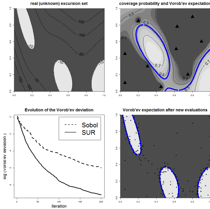
Fig. 2: Top left: Level set of a 2d function. Top right: Coverage probability function after 10 evaluations of f . The Vorob'ev expectation is delimited by the sharp blue line. Bottom left: Decrease of the Vorob'ev deviation when new points are added (2 strategies). Bottom right: New Vorob'ev expectation (SUR strategy)
