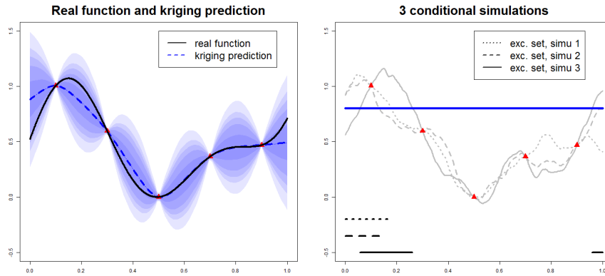
Fig. 1: Conditional simulations of level sets. Left: Kriging model obtained from five evaluations of a 1d function. Right: Three GP conditional simulations, leading to three different level sets. Here the threshold is fixed to T = 0.8 .
