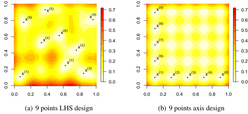
Fig. 1 MSE for two 9-point designs. The univariate kernels are Matérn 5/2 with parameters \sigma^2 = 1 , \theta = 0.2 . For the (scrambled) LHS, the IMSE is I = 0.196 whereas for the axis design I = 0.116 .
