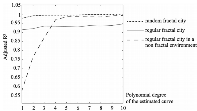
Figure 4. Adjusted R^2 for the series of polynomial estimations of the dilation curve.
