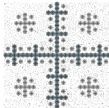
(c) Regular fractal city in a non fractal environment
