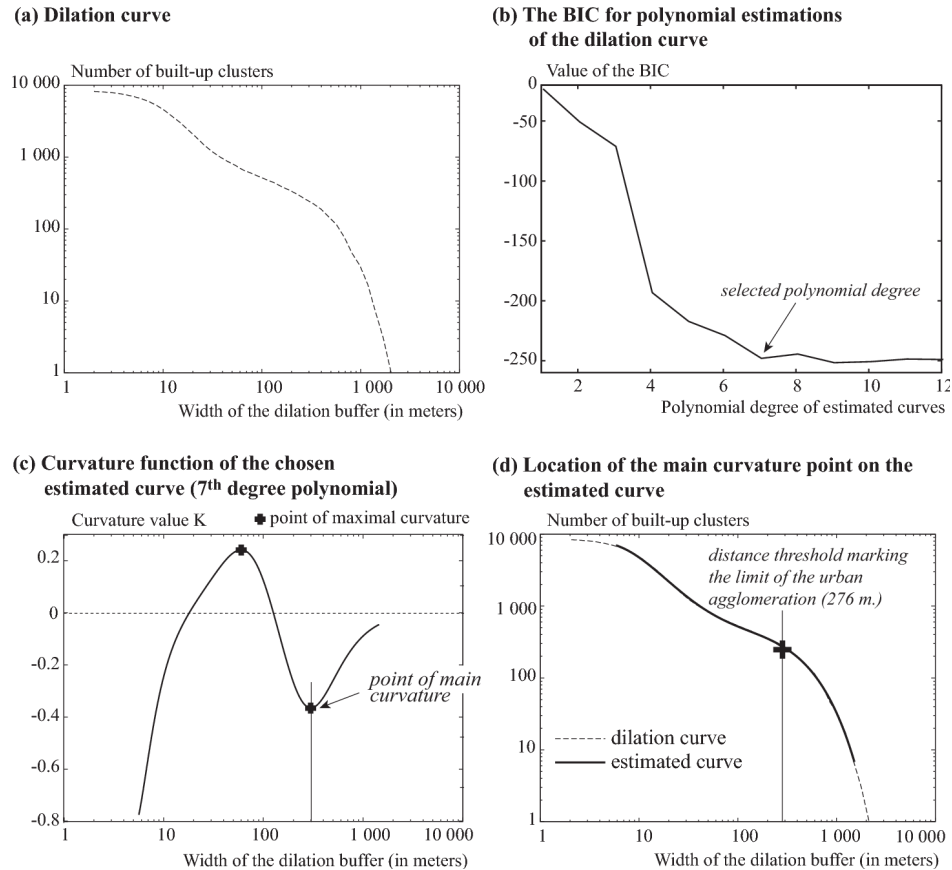
Figure 2. Identification of a significant threshold on the dilation curve (the metropolitan area of Besançon, France example).
